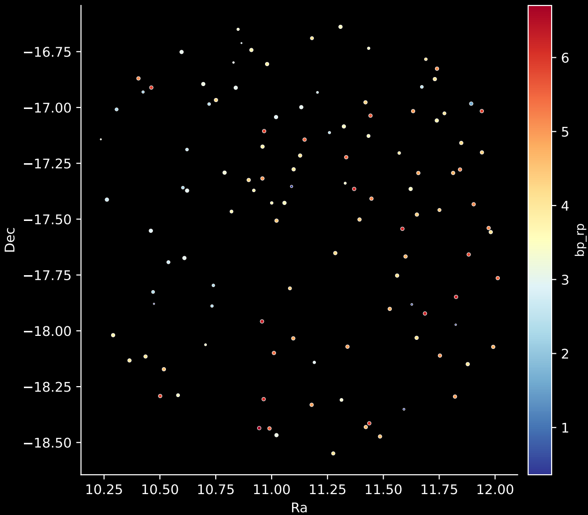
APOGEE DR17 Field: [012+02] Stars: 117
