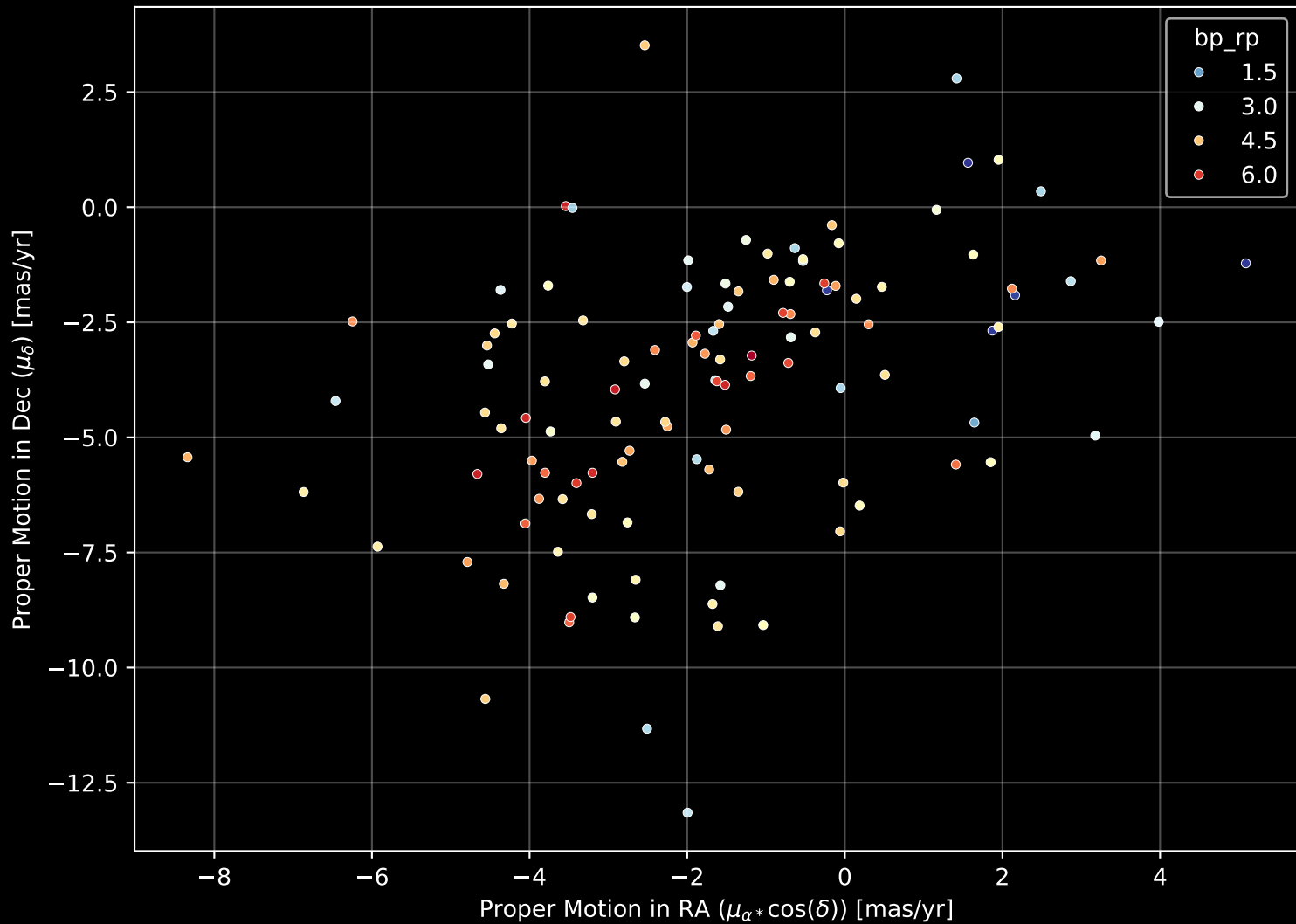
APOGEE DR17 Field: [012+02] Proper Motion Diagram (n= 117)
