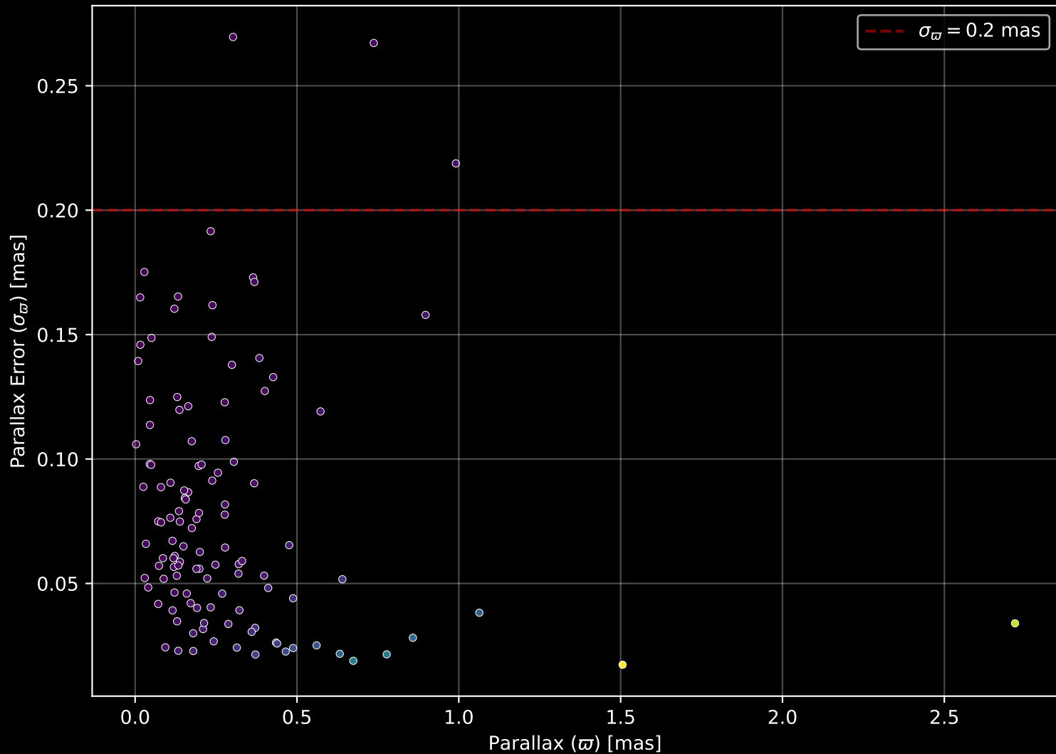
APOGEE DR17 Field: [012+02] Parallax Quality (n= 117)
