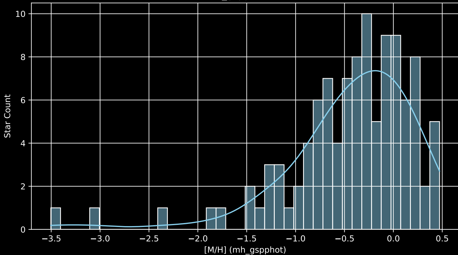
APOGEE DR17 Field: [012+02 [M/H] (mh_gspphot) (n= 107)
