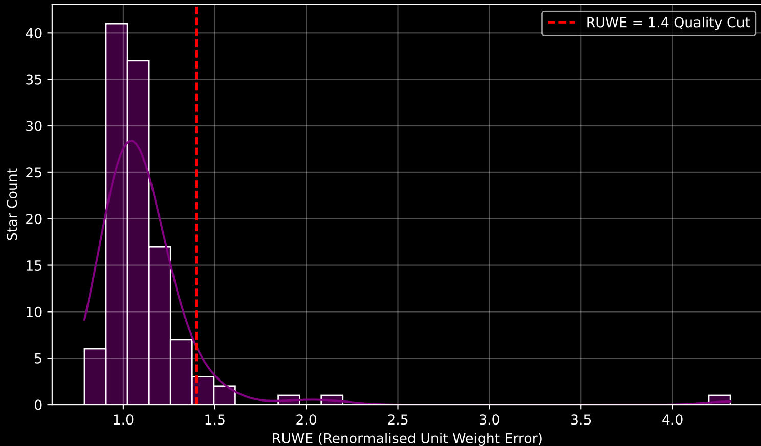
GAPOGEE DR17 Field [012+02] RUWE Distribution (n= 116)
