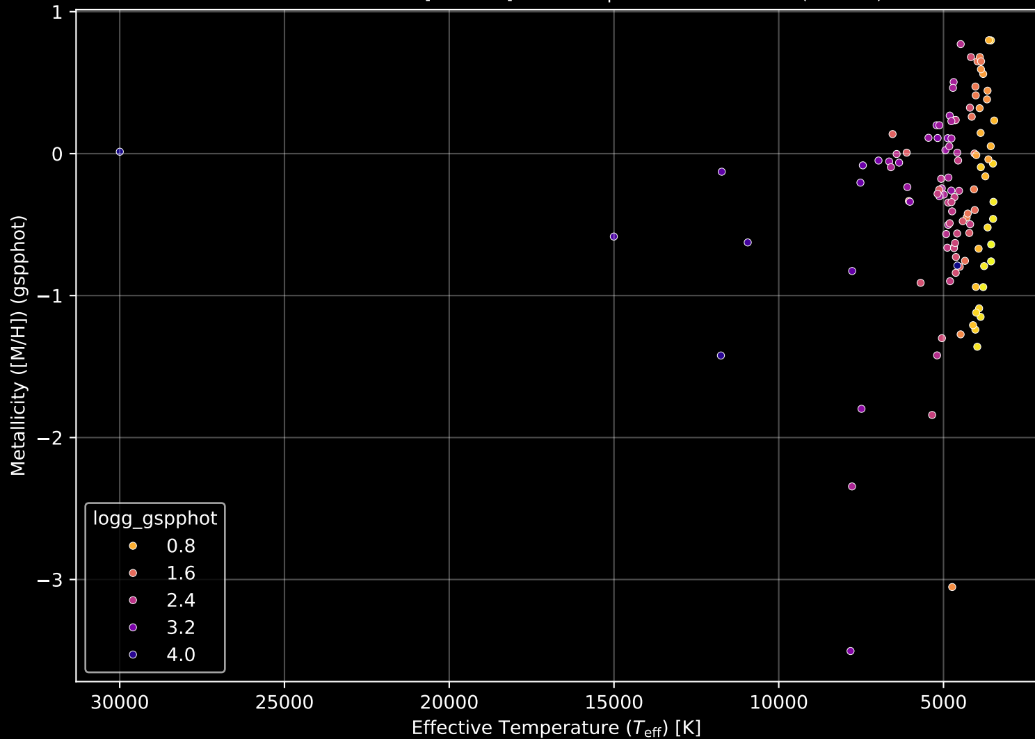
APOGEE DR17 Field: [012+02] Stellar Population Parameters (n= 117)
